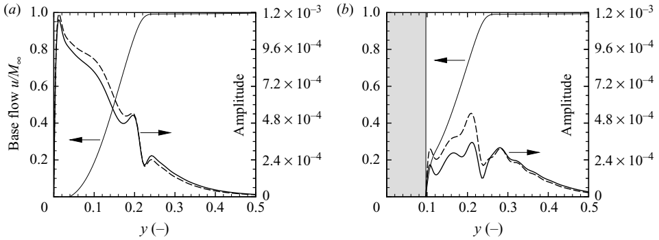
FIGURE 22. Wall-normal amplitude functions |\hat{u}_1| for the forcing frequency F = 1.0 \times 10^{-4} for an isothermal (—) and adiabatic (— · —) boundary condition for the disturbance, roughness with h_R = 0.1 and l_R = 0.4 . The base-flow profile (streamwise velocity) is given for reference. (a) R_x = 1200 . (b) R_x = 1220 .
