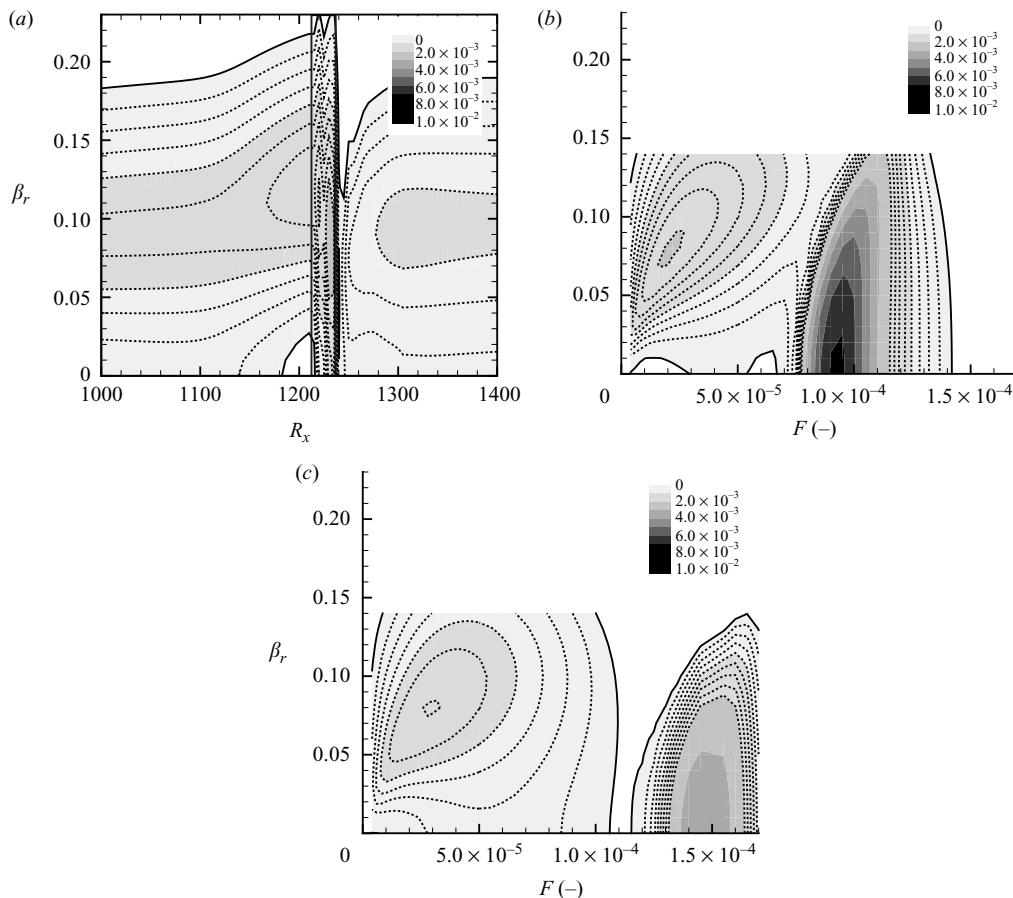
FIGURE 6. Stability diagrams for varying spanwise wavenumbers \beta_r = 2\pi/\lambda_z \times R_x/(Re_\infty M_\infty) . While the greyscales are the same as in figure 5, the contour lines span an interval 0 to 0.005 with \Delta = 0.00025 . (a) F = 0.5 \times 10^{-4} , roughness with h_R = 0.1 and l_R = 0.4 . (b) R_x = 1180 , roughness h_R = 0.1 , l_R = 0.4 . (c) R_x = 1180 , flat plate.
