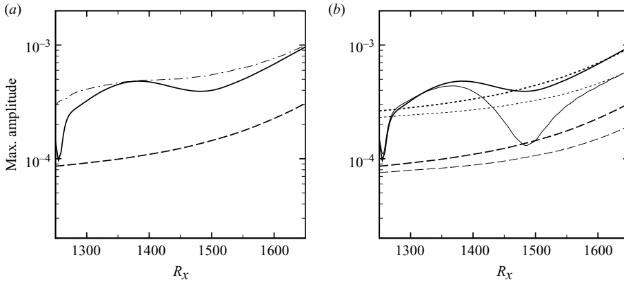
FIGURE 13. Streamwise evolution of the maximum amplitude in the Navier–Stokes simulation with forcing at F = 1.0 \times 10^{-4} : temperature 0.1 \times \hat{T}_1^{max} (— · — · —), streamwise velocity \hat{u}_1^{max} with (—) and without (---) roughness. The roughness with h_R = 0.1 and l_R = 0.4 is located slightly upstream of the depicted streamwise range of R_x . (a) Isothermal BC. (b) Adiabatic BC. Dotted lines (· · · · ·) correspond to \hat{u}_1^{max} for a flat plate, but are shifted by a factor of 3.06.
